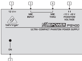
Fig. 1: PS400 connectors and control elements V 1.0
